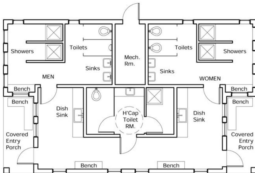
NOBLE VIEW BATH HOUSE FLOOR PLAN
